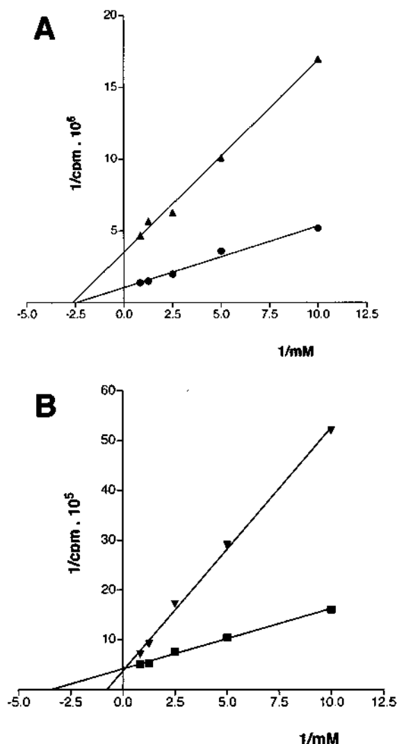
FIGURE 4: Variable inhibition of CK1 activity by peptide AL-9 derived from the NF-AT4 A2 domain. Increasing amounts of (A) inhibitor2-derived RRRKHAAGDDDDAYSITA peptide and of (B) peptide ALZ-1 were phosphorylated as described in the Experimental Section in the absence and in the presence of 40 and 200 \mu M AL-9 peptide, respectively. Shown are the double-reciprocal plots of the data calculated according to Lineweaver–Burk.
