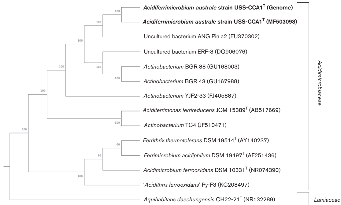
Fig. 1. Consensus phylogenetic tree derived from 16S rRNA gene sequence data showing the relationship of Acidiferrimicrobium australe USS-CCA1 T (MF503098) to other acidophilic representatives of the Acidimicrobiales order. Bootstrap values are indicated at the respective nodes. Aquihabitans daechungensis CH22-21 T (NR132289), a member of the family Lamiaceae was used as outgroup to root the tree. Individual trees used to infer the depicted consensus tree are shown in Fig. S4.
